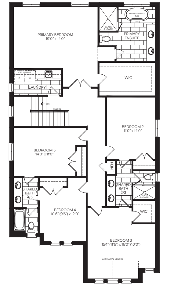
Second Floor Optional 5 Bedroom Plan Elevation A
