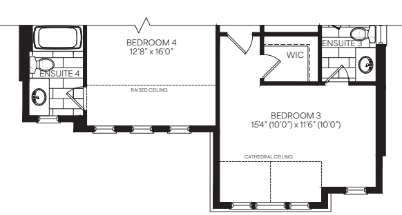
Second Floor Optional 5 Bedroom Plan Elevation B
