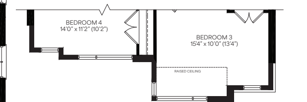
Second Floor Optional 5 Bedroom Plan Elevation C
