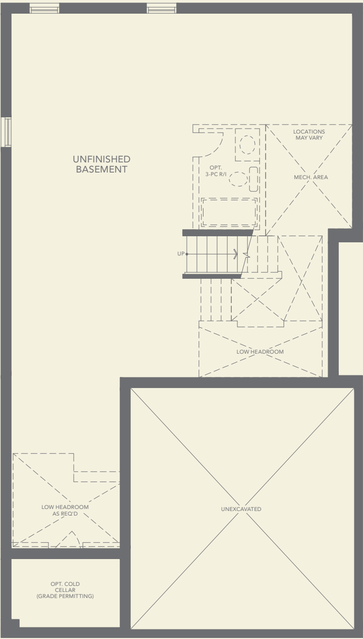
BASEMENT PLAN / ELEVATION C
