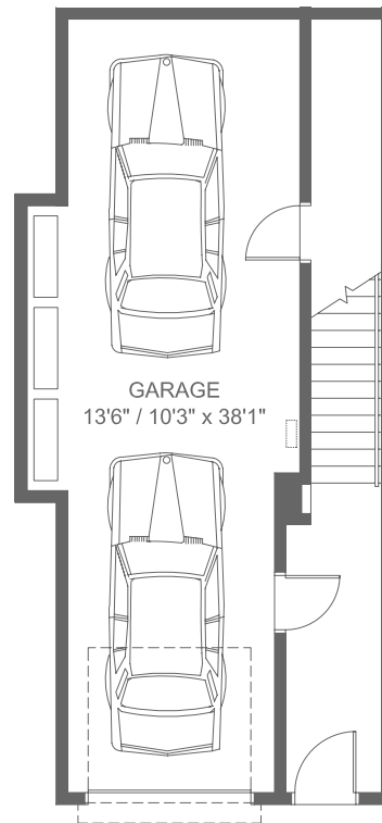
Ground Floor 88 SQ FT
