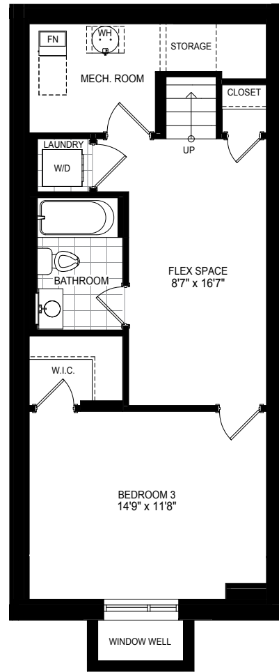
LOWER LEVEL
