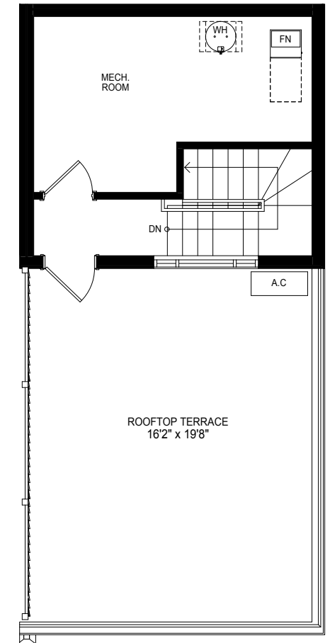
PENTHOUSE FLOOR
