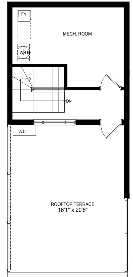
PENTHOUSE FLOOR
