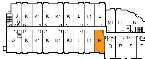
THIRD FLOOR
