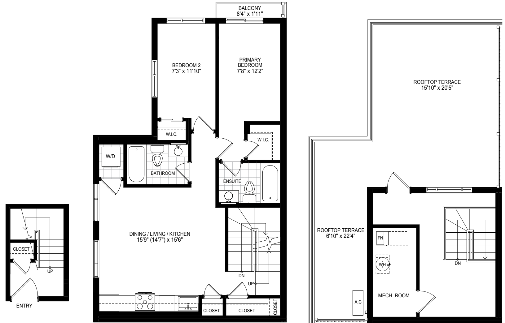
THIRD FLOOR
