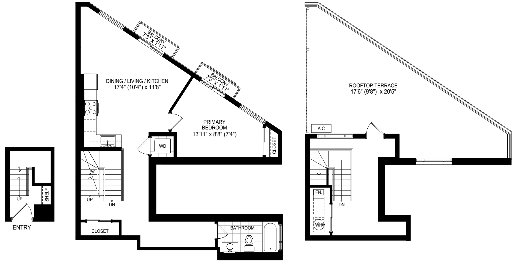
THIRD FLOOR FOURTH FLOOR
