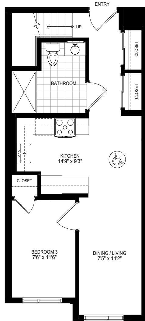
THIRD FLOOR
