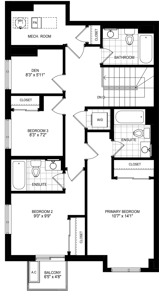
SECOND FLOOR
