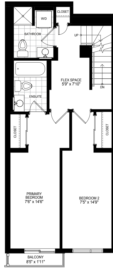
FOURTH FLOOR
