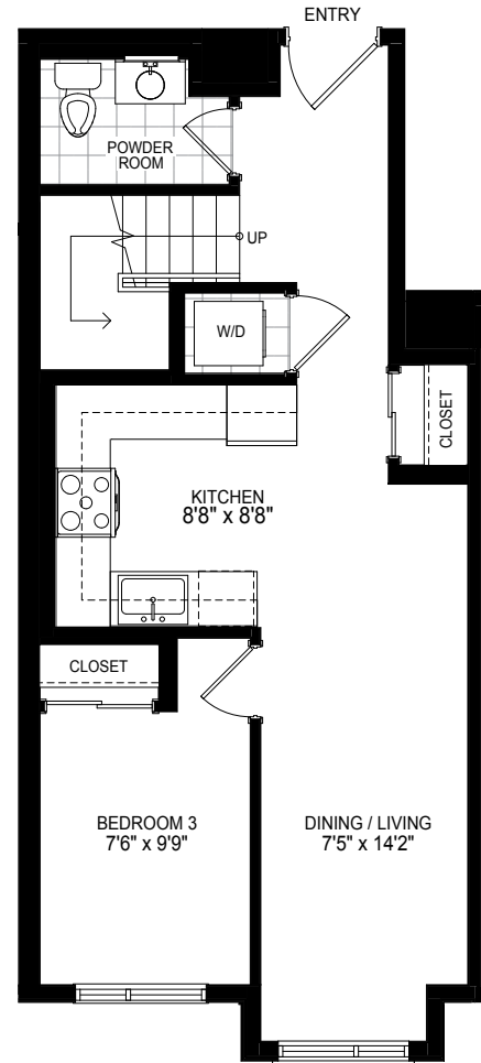
THIRD FLOOR
